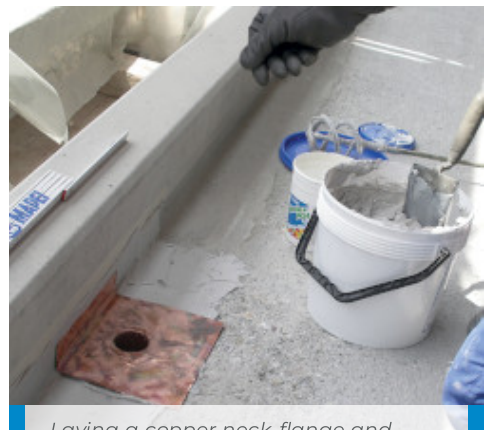
Laying a copper neck-flange and drain spout
